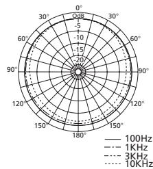
Directivity Characteristics
