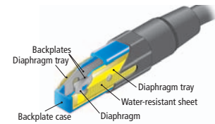
Dual-Diaphragm Mechanism
